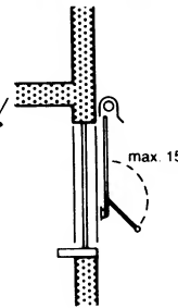
⑰ Partially angled blind
